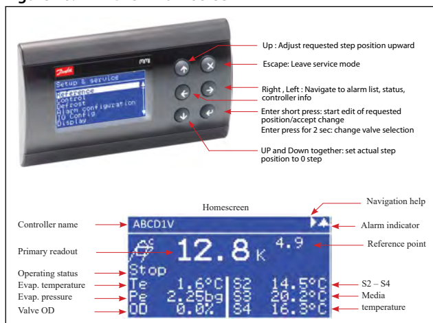
Figure 18: MMIGRS2 Main screen
