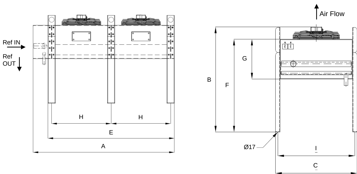
Vertical Mount - Dimension Diagram: KAB01V
