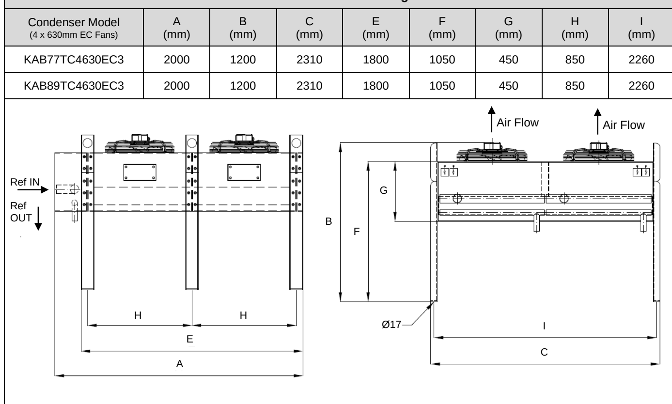
Horizontal Mount - Dimension Diagram: KAB05H
