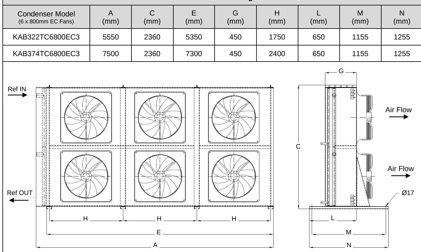
Vertical Mount - Dimension Diagram: KAB9V
