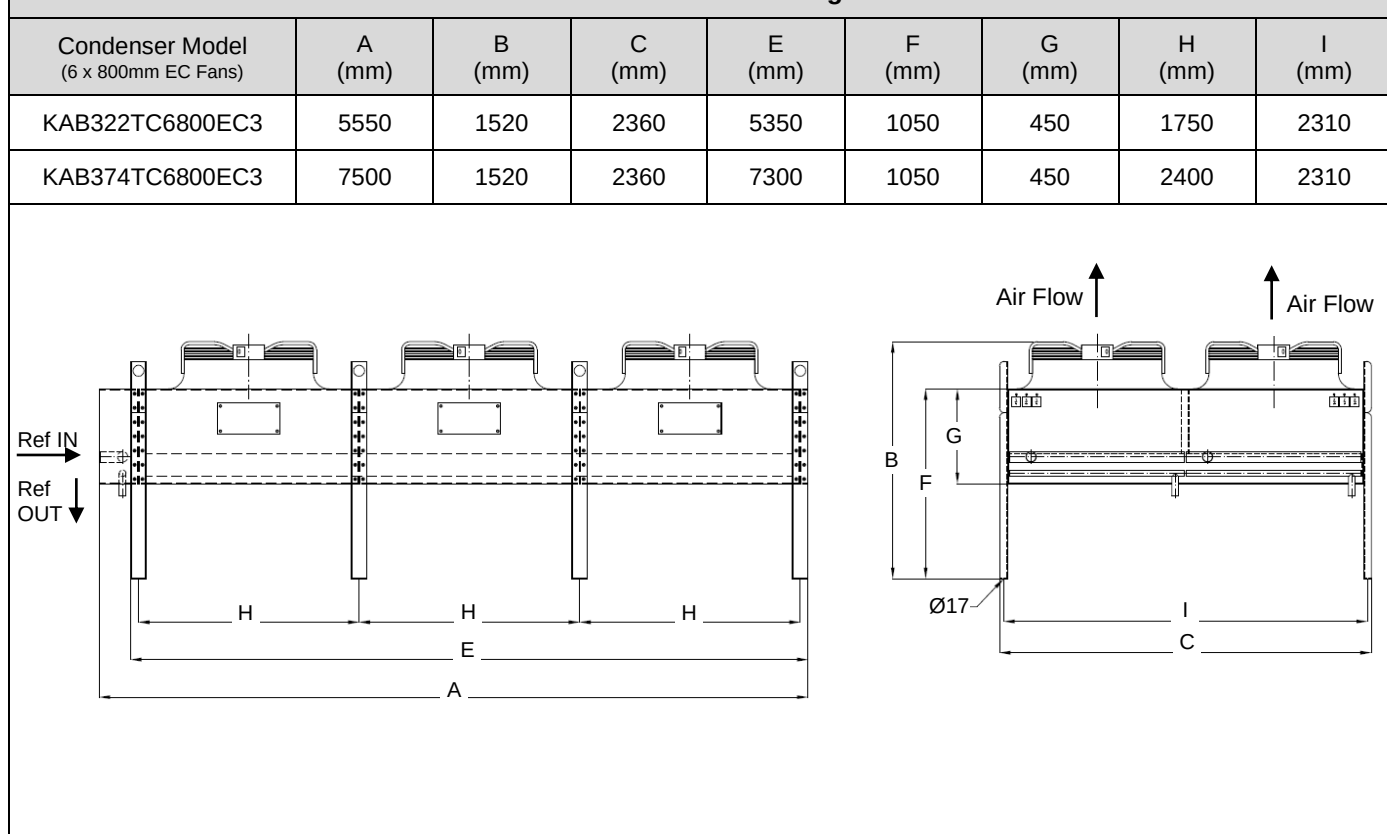
Horizontal Mount - Dimension Diagram: KAB09H
