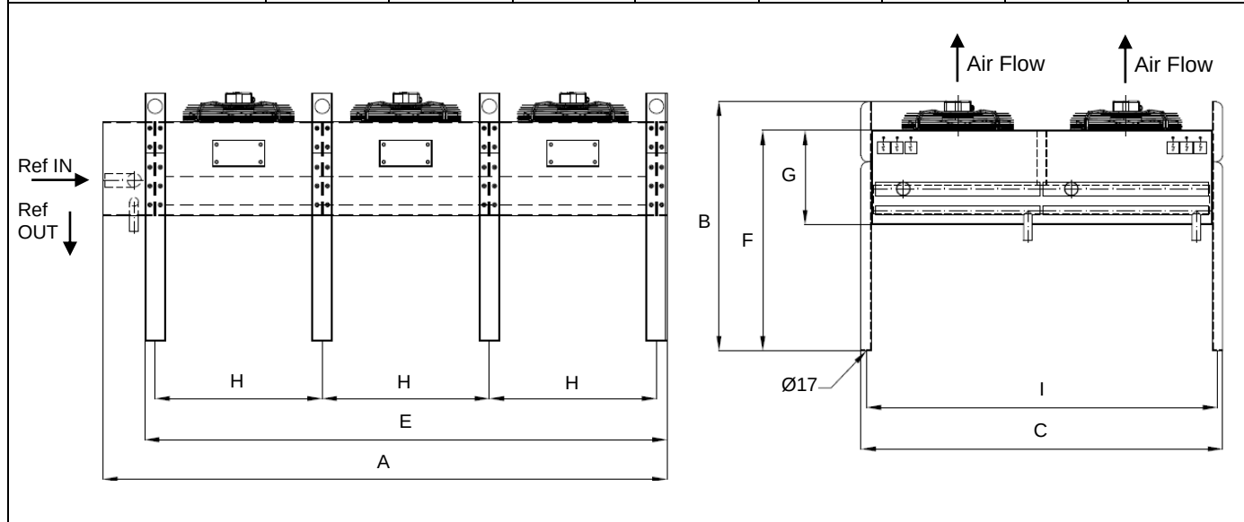
Vertical Mount - Dimension Diagram: KAB06V
