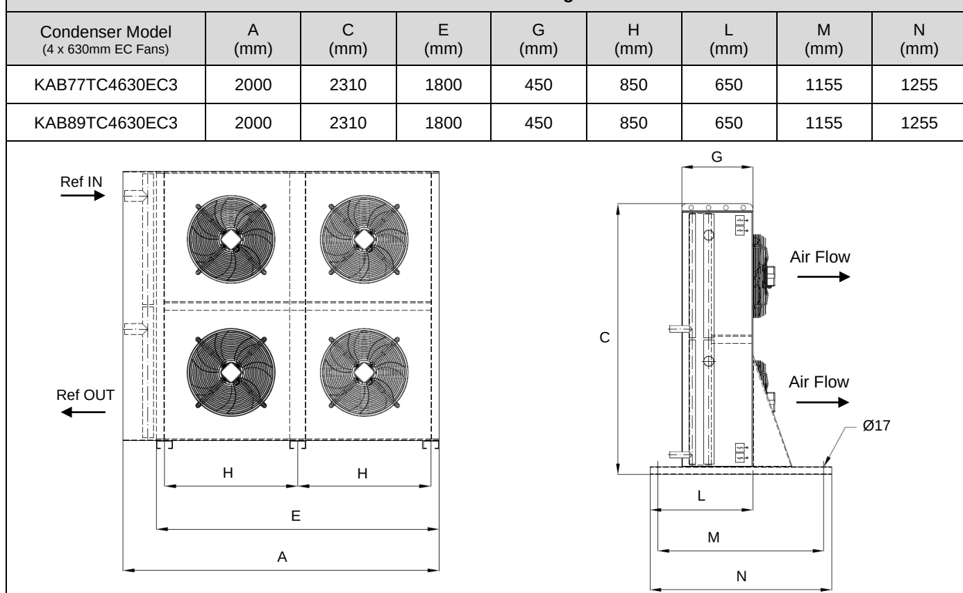
Vertical Mount - Dimension Diagram: KAB05V
